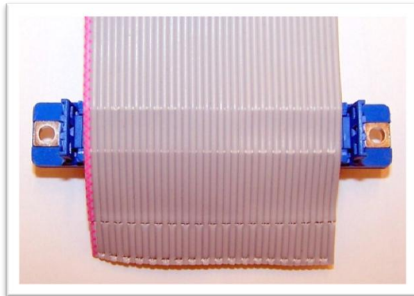
Figure 8: This cable has been flipped and positioned for crimping
